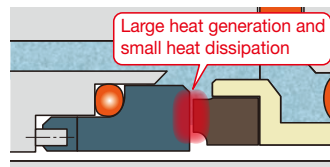
General mechanical seal
