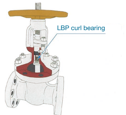
Image of LBP curl bearing mounted on bearing
